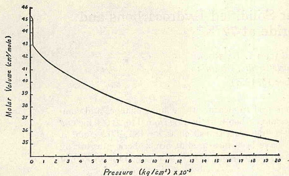
FIG. 1. The molar volume of carbon tetrafluoride at 77°K.
